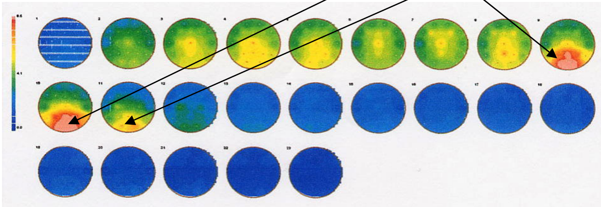
Fig: 5. Topographic Map Displayed in 1 Hz Frequency Bands with Eyes Open, from the First EEG. There is 9-11 Hz dominant frequency activity in posterior regions, with the voltage set at 8.5 \mu V.
